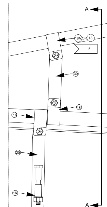
DETAIL A LH SIDE
