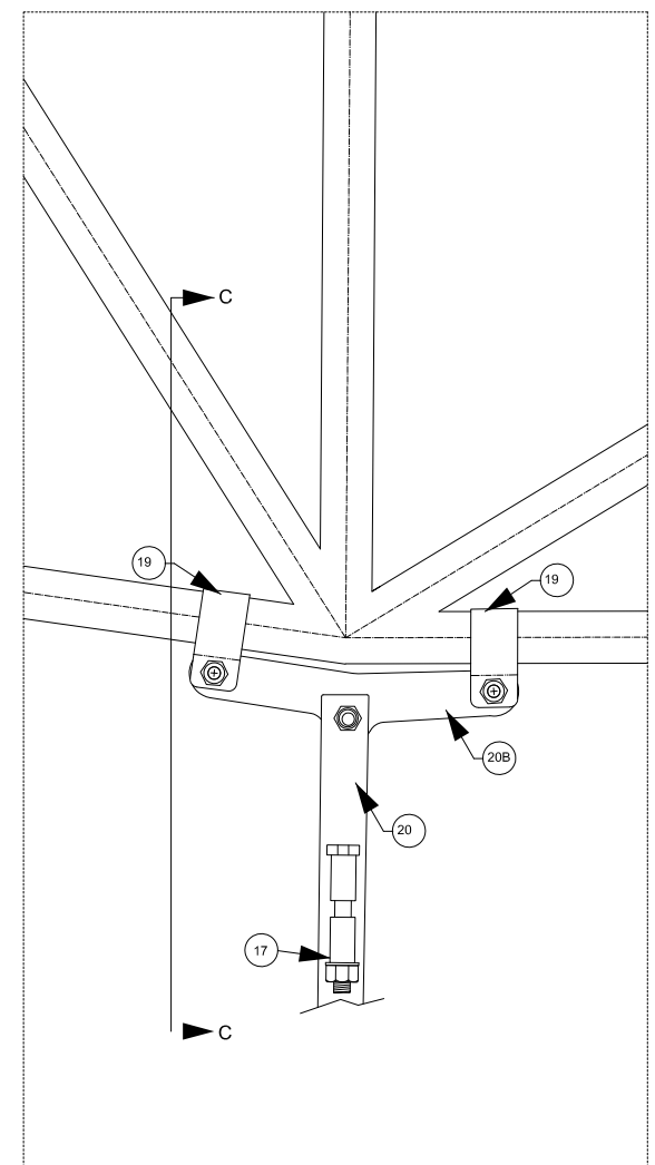
2 DETAIL B RIGHT HAND 4 DEPICTED LH OPOSITE
