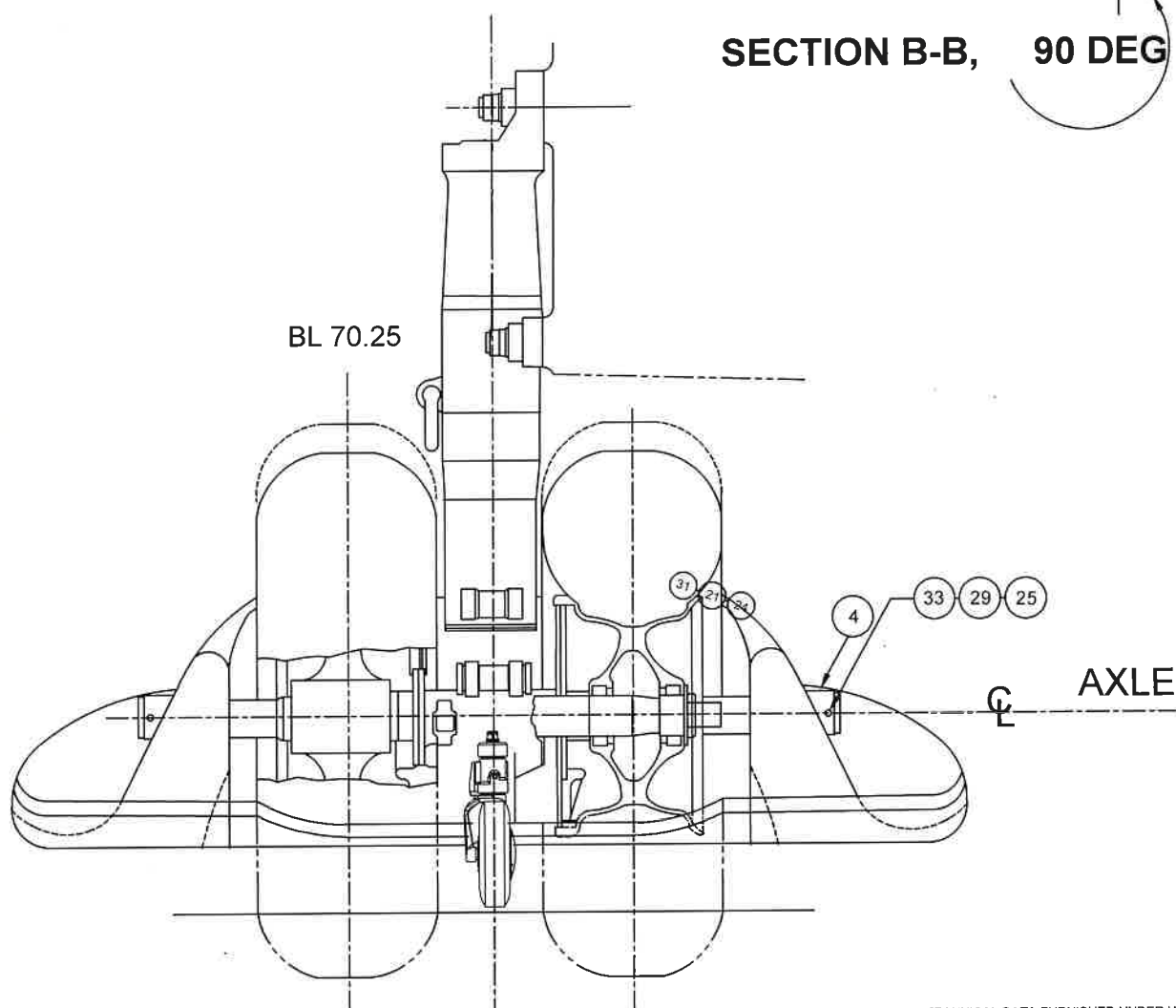
END VIEW LOOKING FWD- FWD L.H. SKI
